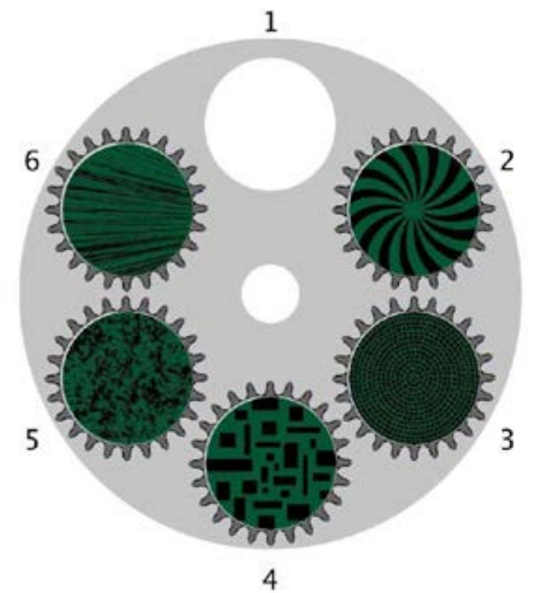
VL1000 WHEELS
